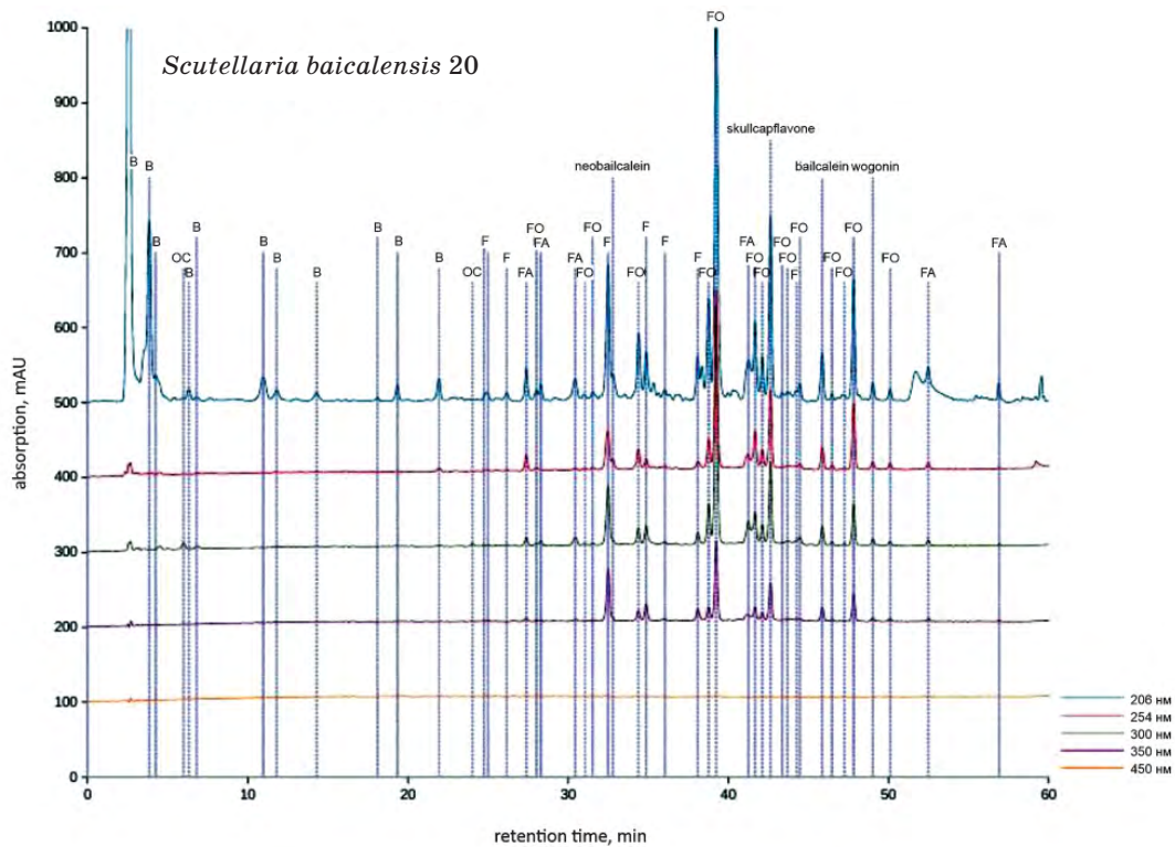
Fig. 5. Chromatographic profiles of dry biomass extract of strain 20SB4 of S. baicalensis plant tissue culture Labels of substances: A — unrestrained pool of hydrophilic substances (free organic acids, amino acids, etc.) + solvent; B — derivatives of benzoic and oxybenzoic acids; OS — derivatives of oxcinnamic acid; F — flavans; FA — flavones; FA — flavones similar to neobaikalein (there are hydroxyls in the phenyl moiety); FO — flavones similar to baicalein and wogonin (without hydroxy fragments); F — other flavonoids; flavones: neobaicalein, skullcapflavone, baicalein, wogonin
