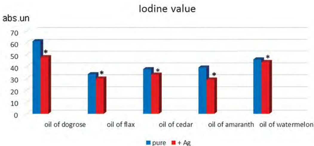
Fig. 2. Iodine value of pure oils and oils with silver nanoparticles
