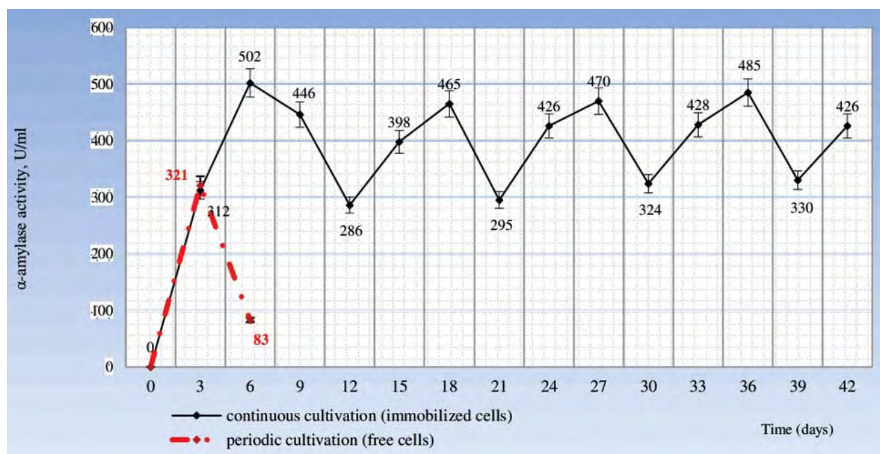
Fig. 3. Alpha-amylase production by immobilized Aspergillus oryzae M
