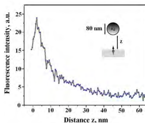
Fig. 4. Single molecule fluorescence rate dependence on the particle-surface distance for an 80 nm silver nanoparticle [48]
