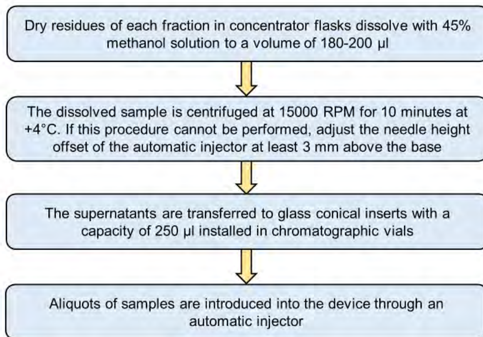
Fig. 5. The procedure steps for performing HPLC/MS analysis
