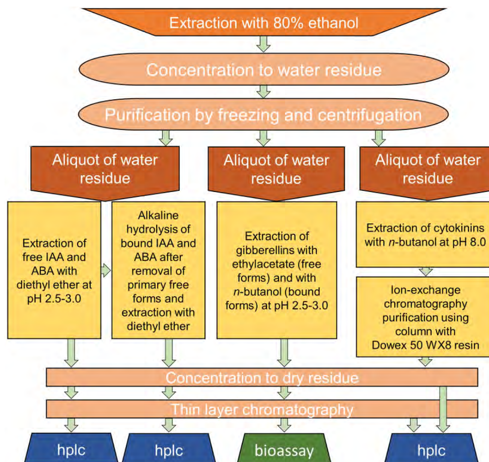
Fig. 1. The regular procedure of isolation, purification, fractionation, and analysis of auxins, gibberellins, cytokinins, abscisic acid in plant tissues: HPLC — high-performance liquid chromatography
