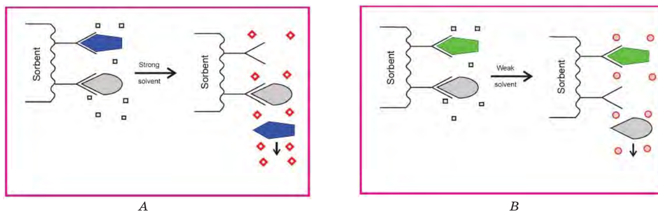
Fig. 4. A simplified scheme of the sample substances separation in the cartridge SPE Oasis MCX, 6 cc/150 mg Waters: A — selective elution of acidic analytes; B — the leaching of pollutants Quantification with HPLC/MS
